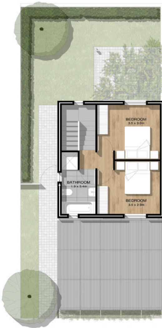
First Storey Plan 1:50
